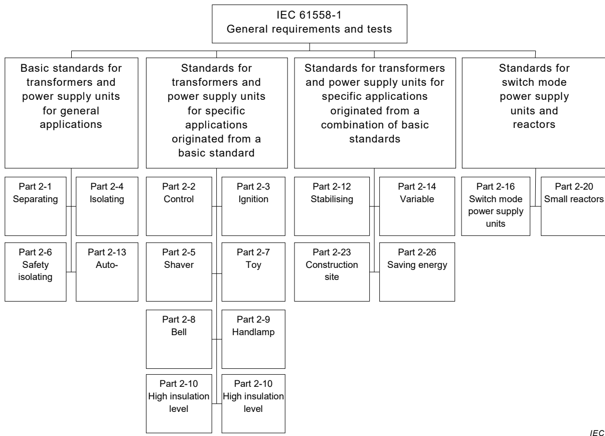
Figure 1 – IEC 61558 principle
