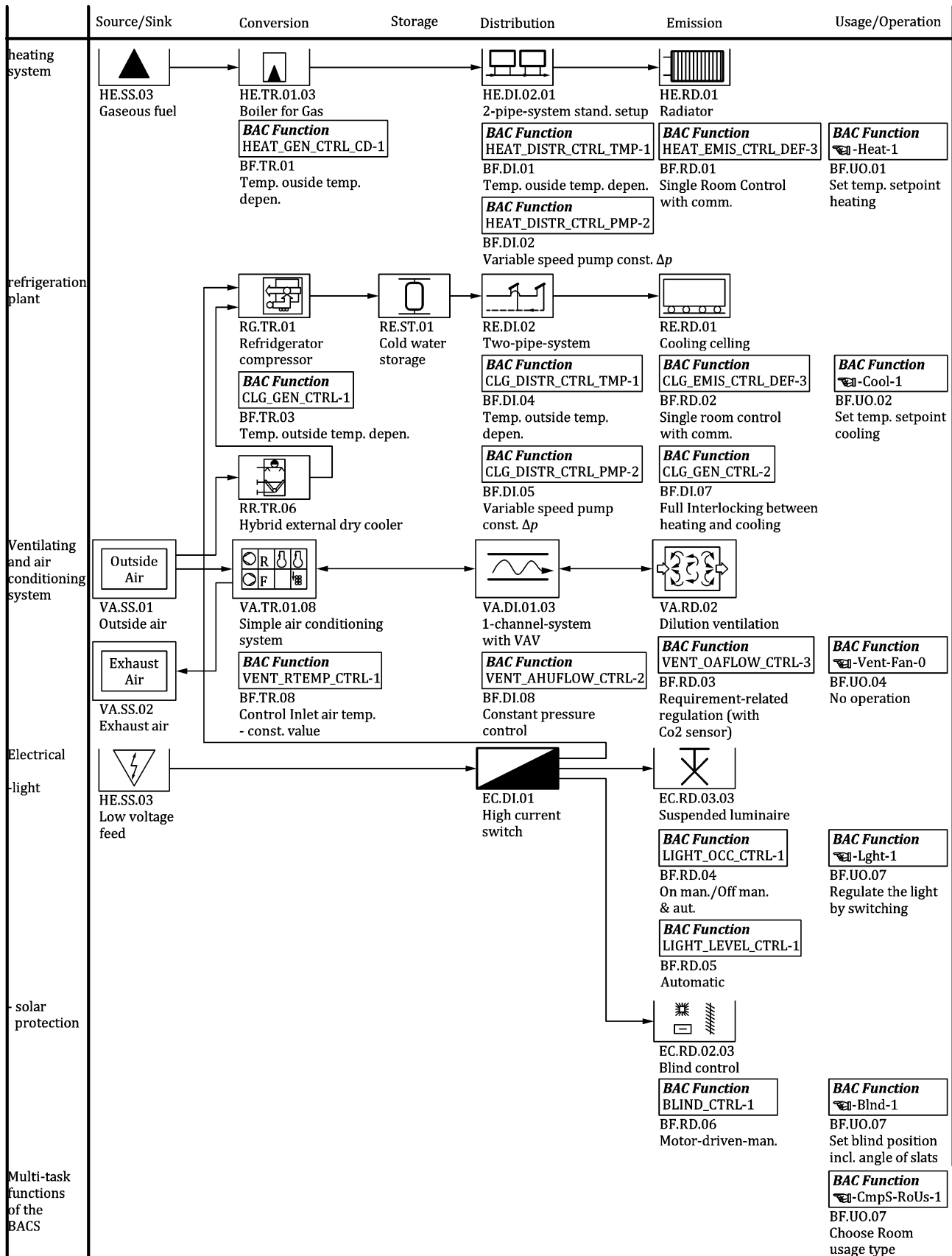
Figure 2 — Example for documentation of design choices for technical infrastructure and associated control functions of a building (Source: SN 502411:2016 / SIA 411:2016)
