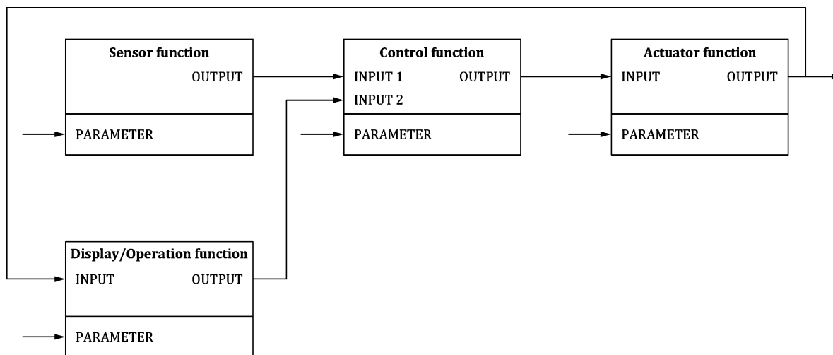
Figure 4 — Relationship between Automation functions (typical example)
