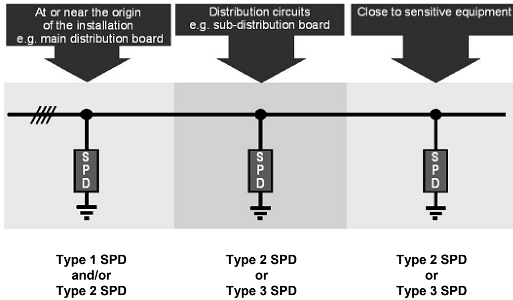
Figure 534.1 — Example of installation of Type 1, Type 2 and Type 3 SPDs
